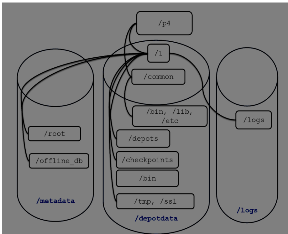
Figure 2: SDP Runtime Structure and Volume Layout
