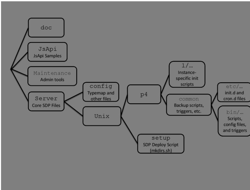
Figure 1: SDP Package Directory Structure
