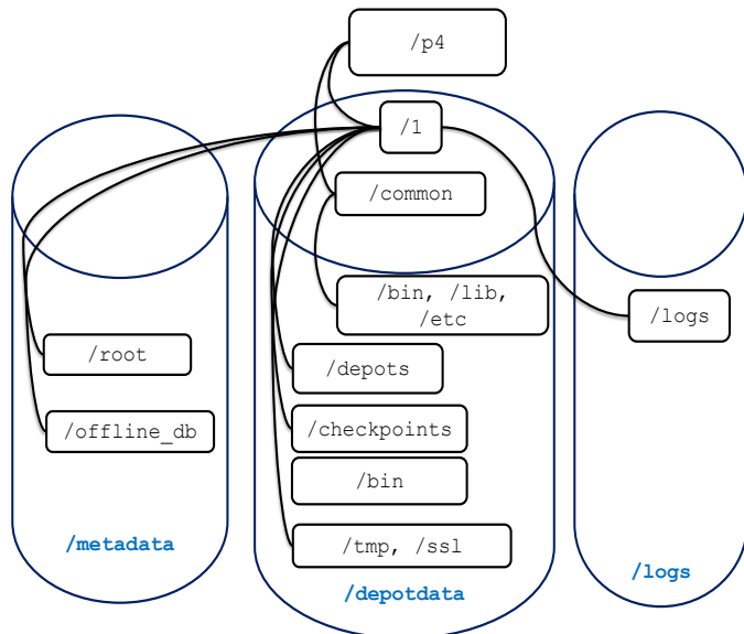
Figure 2: SDP Runtime Structure and Volume Layout
